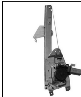
Elevalunas original – lève-vitre original – oem window regulator – levandator de vidro original
