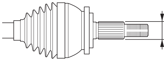
Figure 1: In order to identify the correct wheel bearing, measure the outer diameter of the CV joint splined shaft
